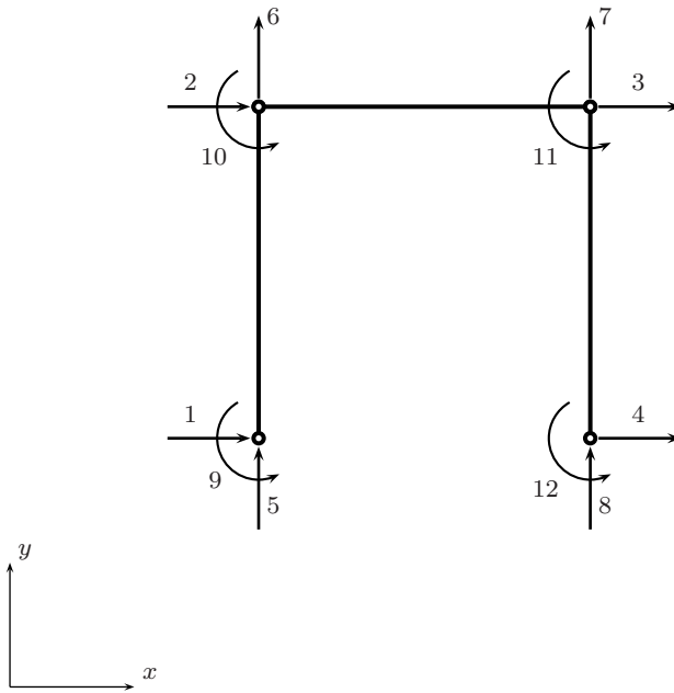
Fig. 7.6 A 2D frame example: degree of freedom ordering
