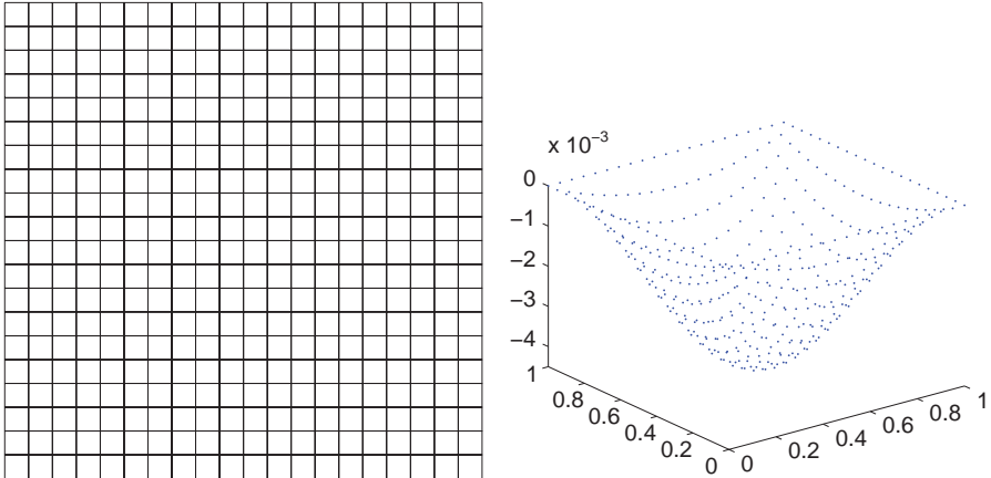
Fig. 12.2 Mesh of 20 \times 20 Q4 elements and deformed shape
